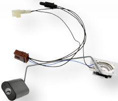
K07013 Fuel Level Sensor Nissan Murano 2009-03 VIO over 485,000
