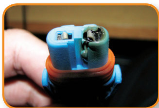
Melted Original-style Unit
